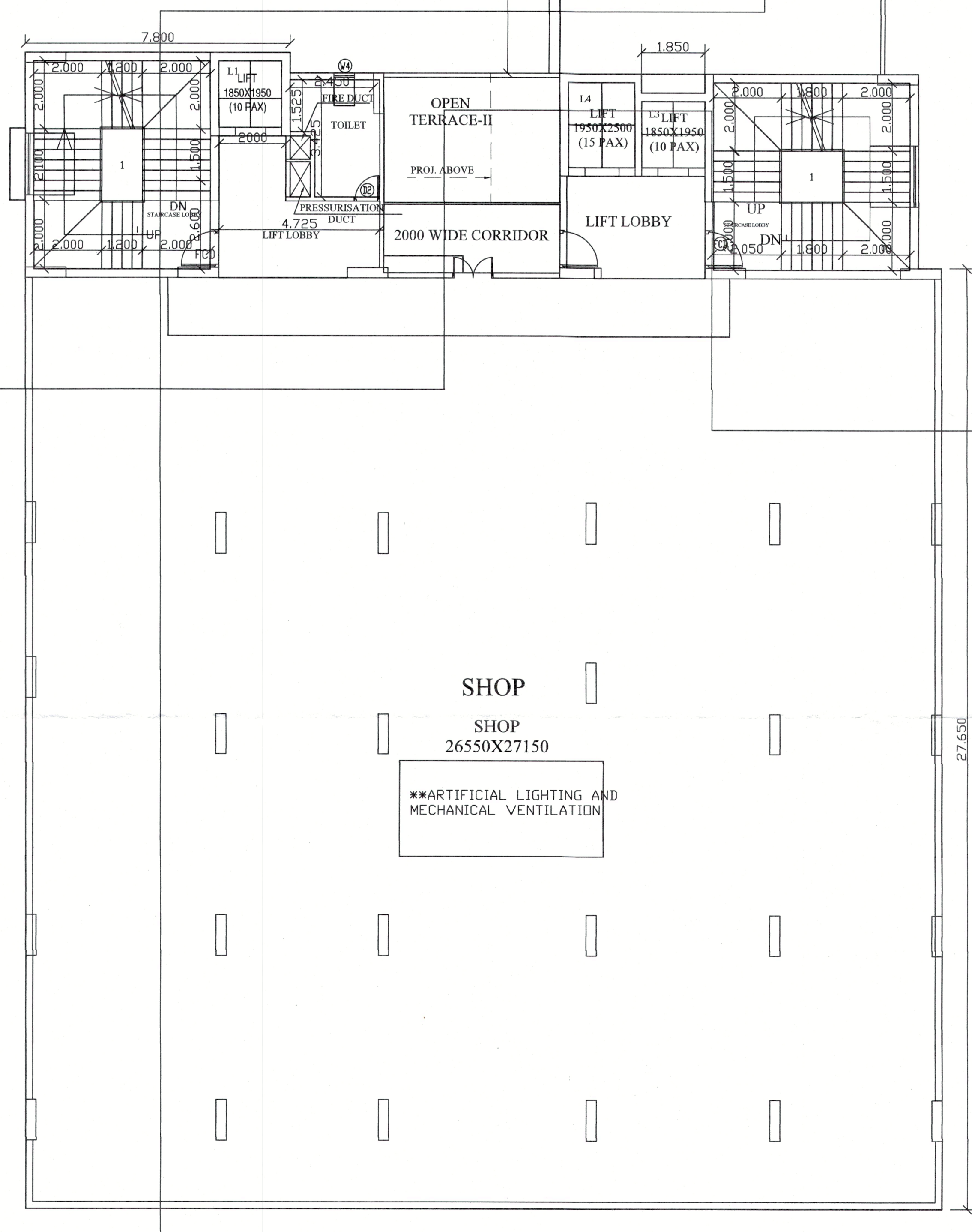
FLOOR01 WING-1 SCALE - 1:1
